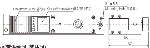
AZL112-K1□L□□-GN-RL5 With Supply Valve And Release Valve(带供给阀 破坏阀)
