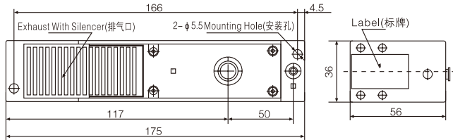
AZL112-GN With Vacuum Adapter(带真空用接头)
